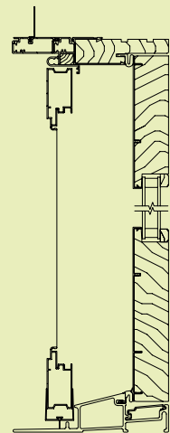
HEAD/SILL SECTION
